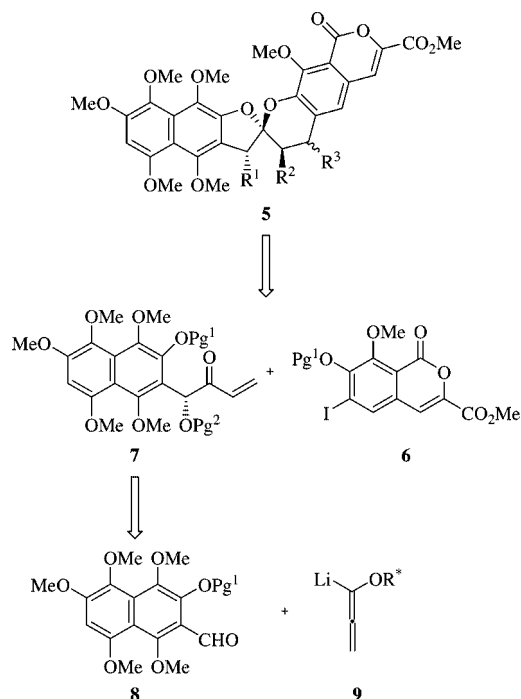
Scheme 1. Retrosynthetic analysis of rubromycins (Pg = protecting group).
