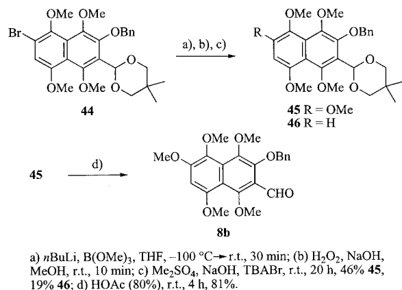
Scheme 14. Synthesis of hexaalkoxy-substituted naphthaldehyde 8b according to Route III.
