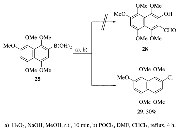
Scheme 9. Attempt to prepare formylated naphthalene derivative 28 .
