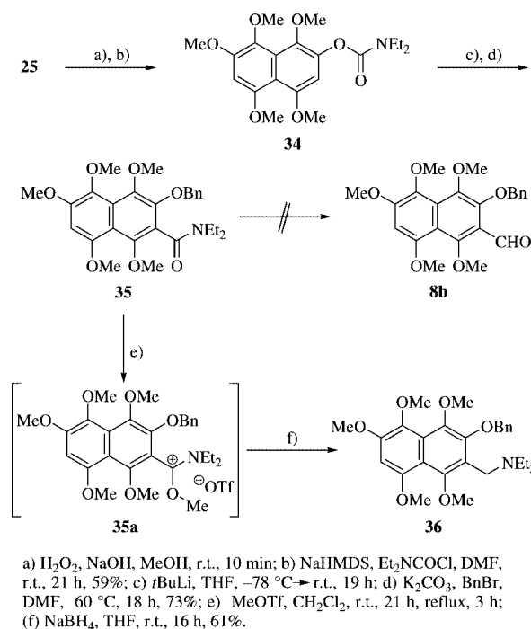
Scheme 11. Synthesis of naphthyl-substituted amide 35 by ortho -Fries rearrangement of compound 34 and its attempted conversions into aldehyde 8b .
