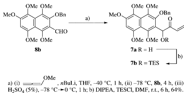
Scheme 15. Synthesis of \alpha -hydroxy enone 7a from key aldehyde 8b and lithiated methoxyallene and its conversion into 7b .
