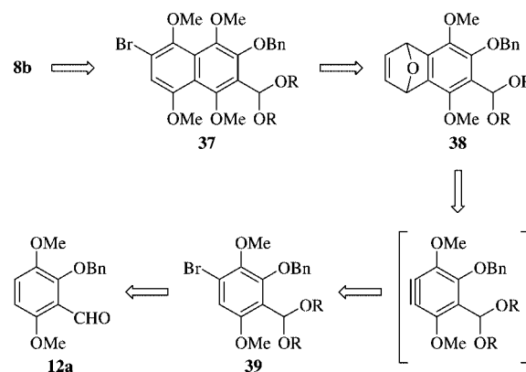
Scheme 12. Retrosynthetic analysis of precursor 37 required for synthesis of aldehyde 8b (Route III).
