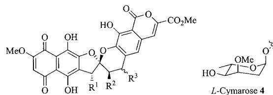
\gamma -Rubromycin 1 : R^1 = R^2 = R^3 = H Purpurumycin 2 : R^1 = R^2 = H , R^3 = OH Heliquinomycin 3 : R^1 = O -Cymarose, R^2 = OH , R^3 = H
