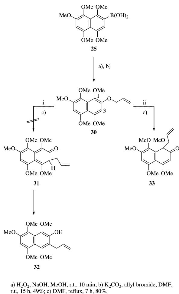
Scheme 10. Synthesis and Claisen rearrangement of O -allylated naphthalene derivative 30 .
