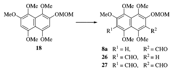
Scheme 8. Synthesis of formylnaphthalene derivative 8a .
