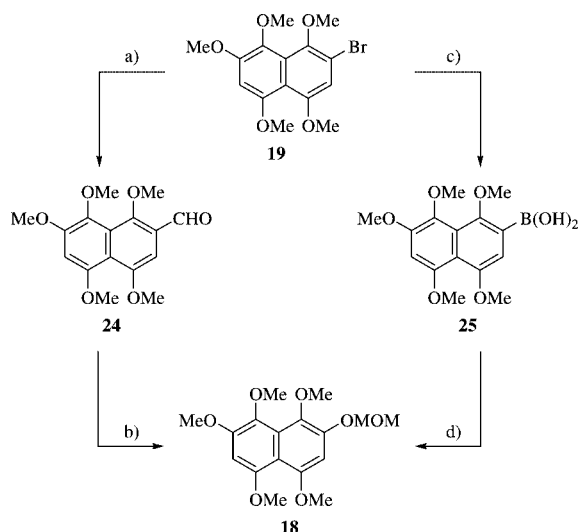
Scheme 8. Synthesis of formylnaphthalene derivative 8a .
