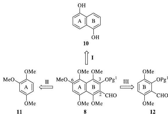
Scheme 2. Retrosynthetic analysis of naphthaldehyde 8 (Routes I, II, III).
