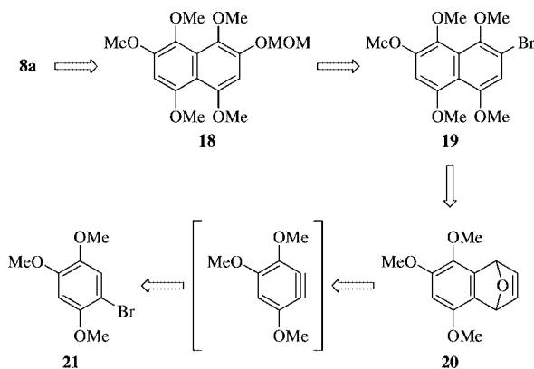
Scheme 5. Retrosynthetic analysis of precursor 18 required for synthesis of 8a (Route II).
